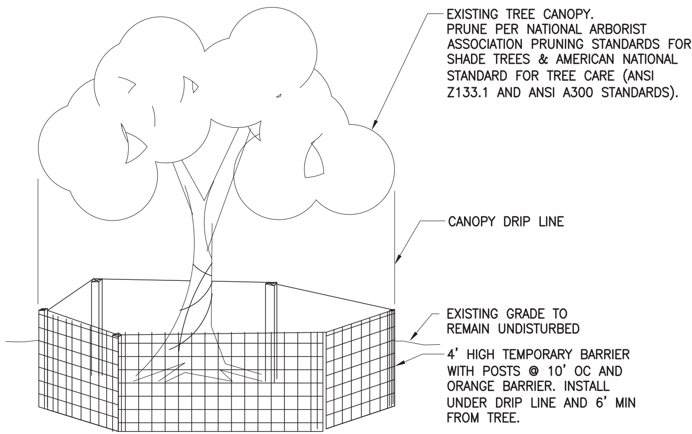
EXISTING VEGETATION PROTECTION DETAIL – PERIMETER PROTECTION ZONE (PPZ)
