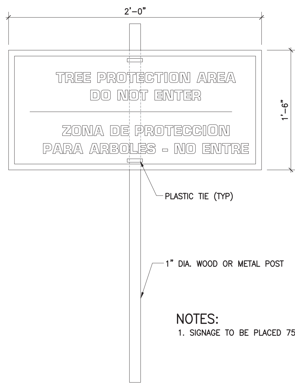
DETAIL – TPA FENCE SIGNAGE
