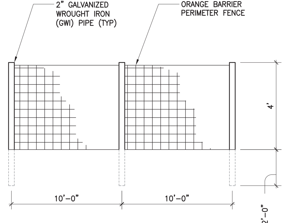
DETAIL – TREE PROTECTION AREA (TPA) FENCE
